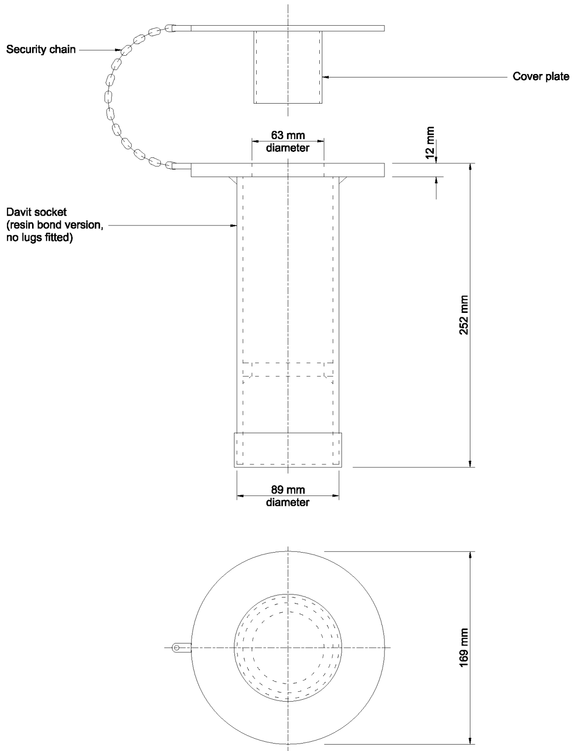
Figure D 1 Standard flush mount davit socket
