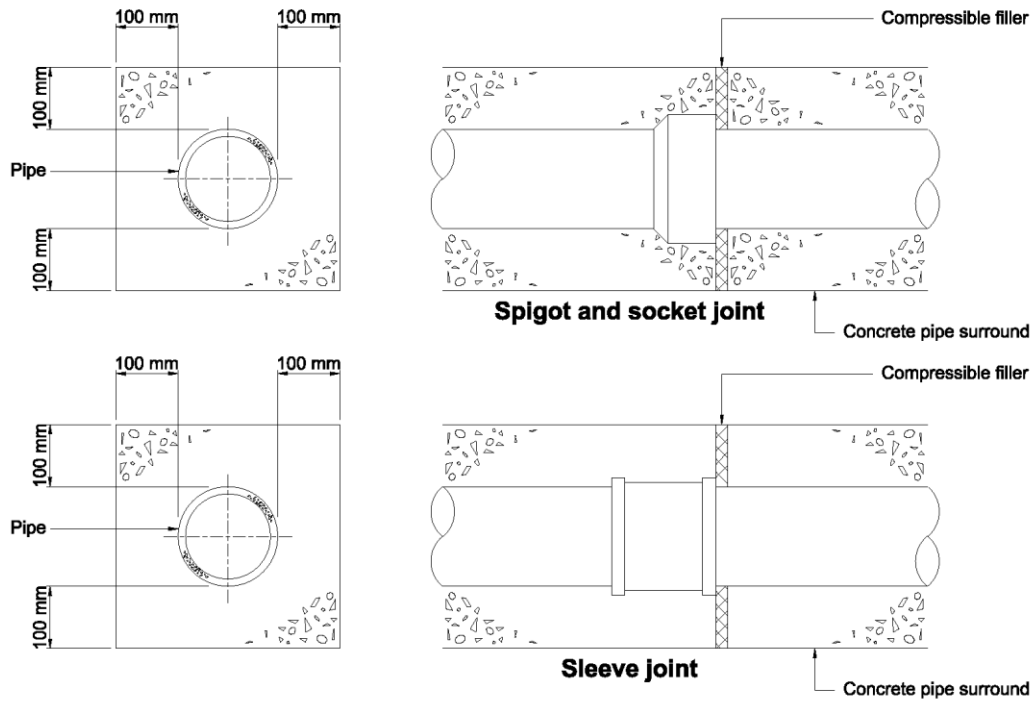
Figure B 28 Joints for encased pipes
