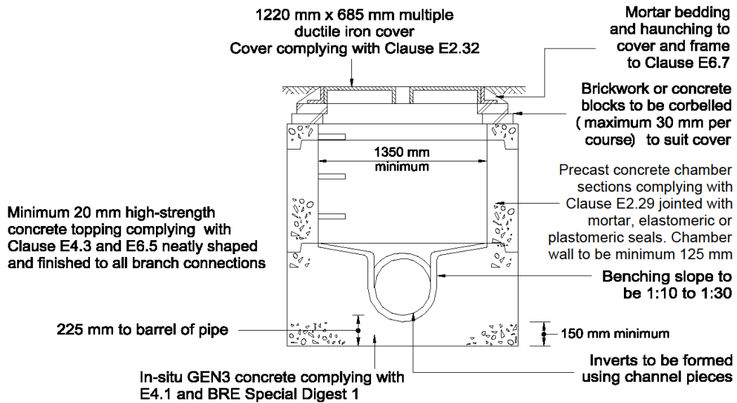
Figure B 15 Typical manhole detail – Type C Depth from cover level to soffit of pipe less than 1.5 m Rigid material construction
